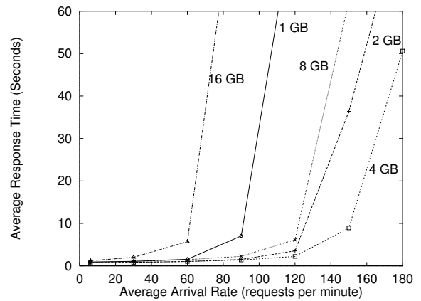
(c) CPU = 4
