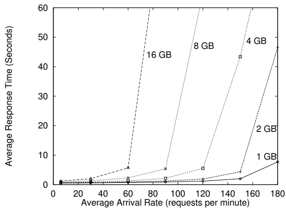
(c) CPU = 4
