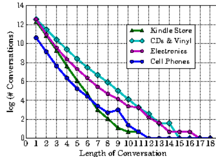
Figure 4: Statistical distribution of the number of conversations over the length of conversations on four datasets.
