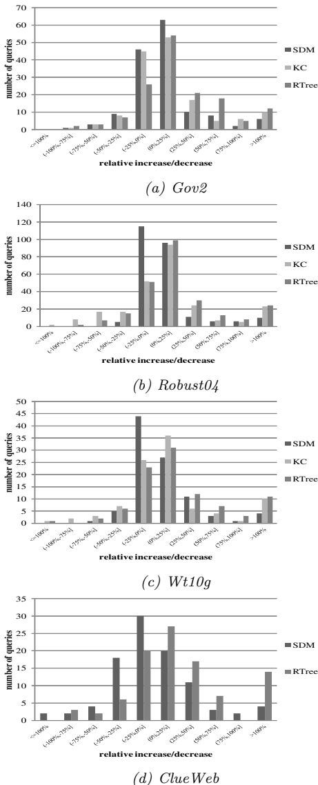
Figure 5: Analysis of relative increases/decreases of MAP over QL using the non-stemmed index.
