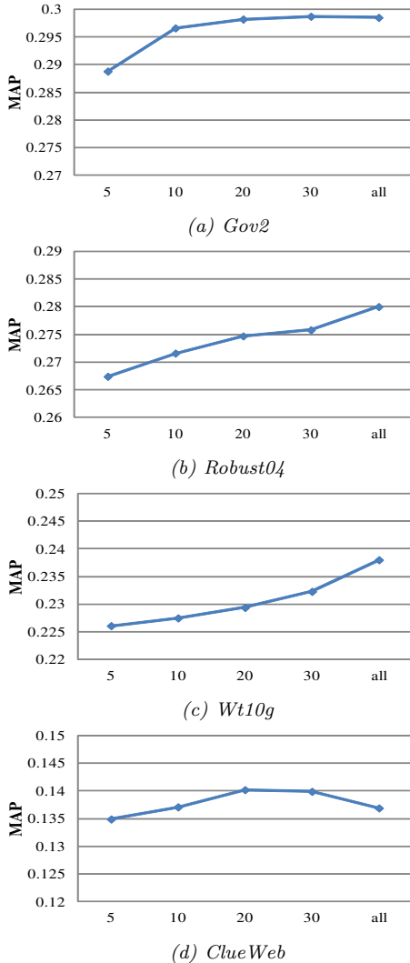
Figure 6: The effect of the parameter SubNum . x-axis denotes SubNum and y-axis denotes MAP.
