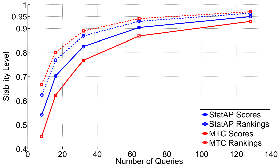
Figure 3: Stability level of MAP scores and induced ranking of systems for statAP and MTC as a function of the number of queries.
