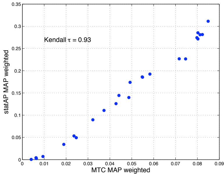
Figure 1: MTC and statAP weighted-MAP correlation
