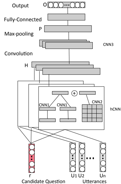
Figure 1: Our proposed multi-turn hybrid CNN.
